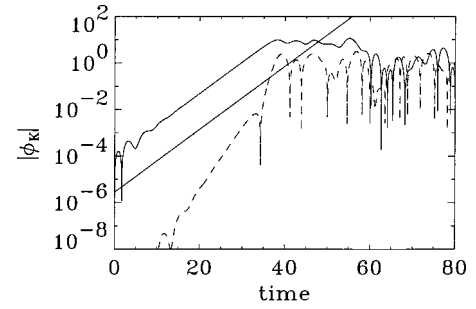
FIG. 5. Two-stream instability—evolution of the fundamental mode K_0=0.8 (solid line) and first harmonic 2K_0 (dashed line) of the electrostatic potential, for H=0.25 . The straight line corresponds to the growth rate of K_0 computed from linear theory, \gamma = 0.3116 .
